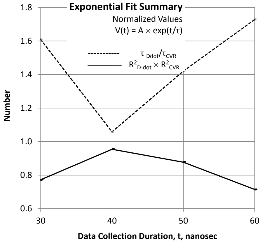
Figure 44. The R^2_{D-dot} \times R^2_{CVR} product and the \tau_{D-dot}/\tau_{CVR} ratio are optimal when equal to unity and most nearly approximate unity at 40 ns.
