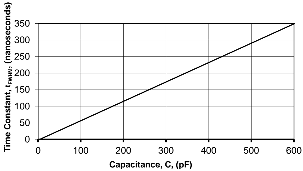
Figure 35. Only the independent C of Equation (27) is varied to see its predicted linear, direct effect on the dependent t_{FWHM} .
